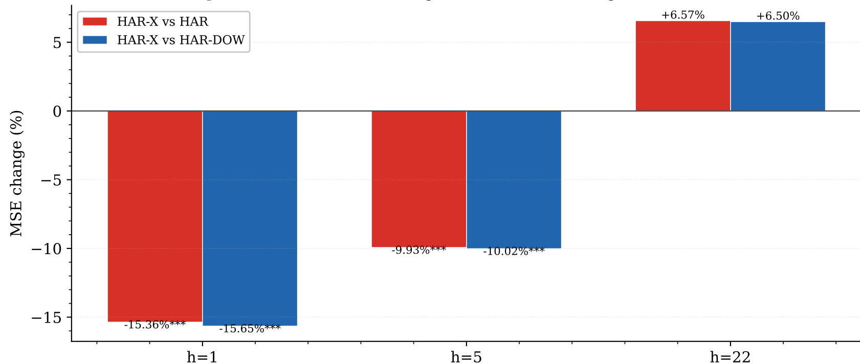
HAR-X out-of-sample MSE vs benchmarks (negative = better; * DM significance)
